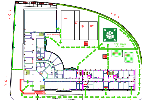
VAZİYET PLANI / SITE PLAN
